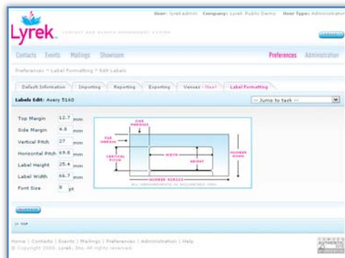
Lyrek Format Avery® Labels
